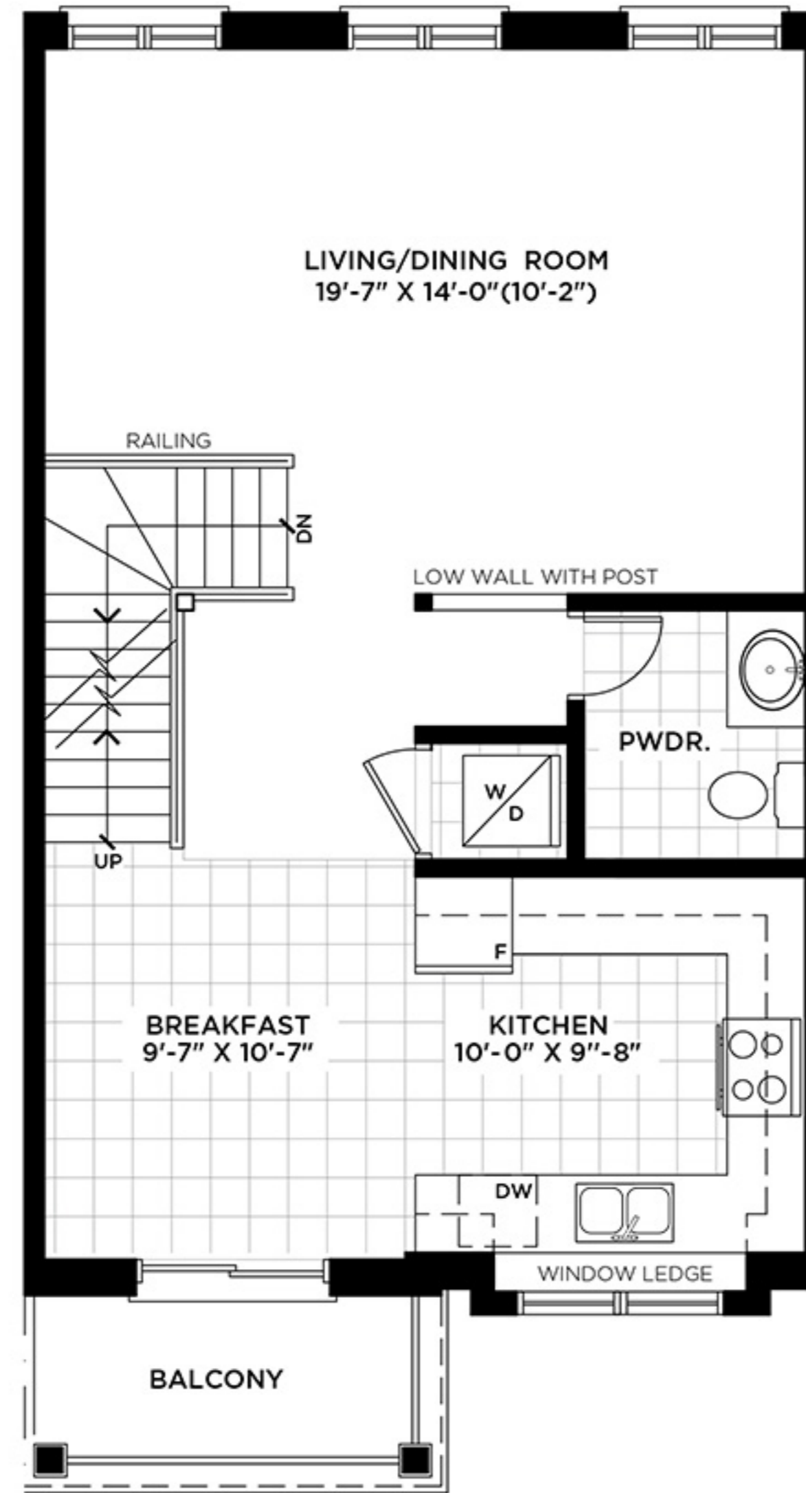
SECOND FLOOR PLAN ELEV. 'B' INT. UNIT 19-24 END UNIT 18, 25
