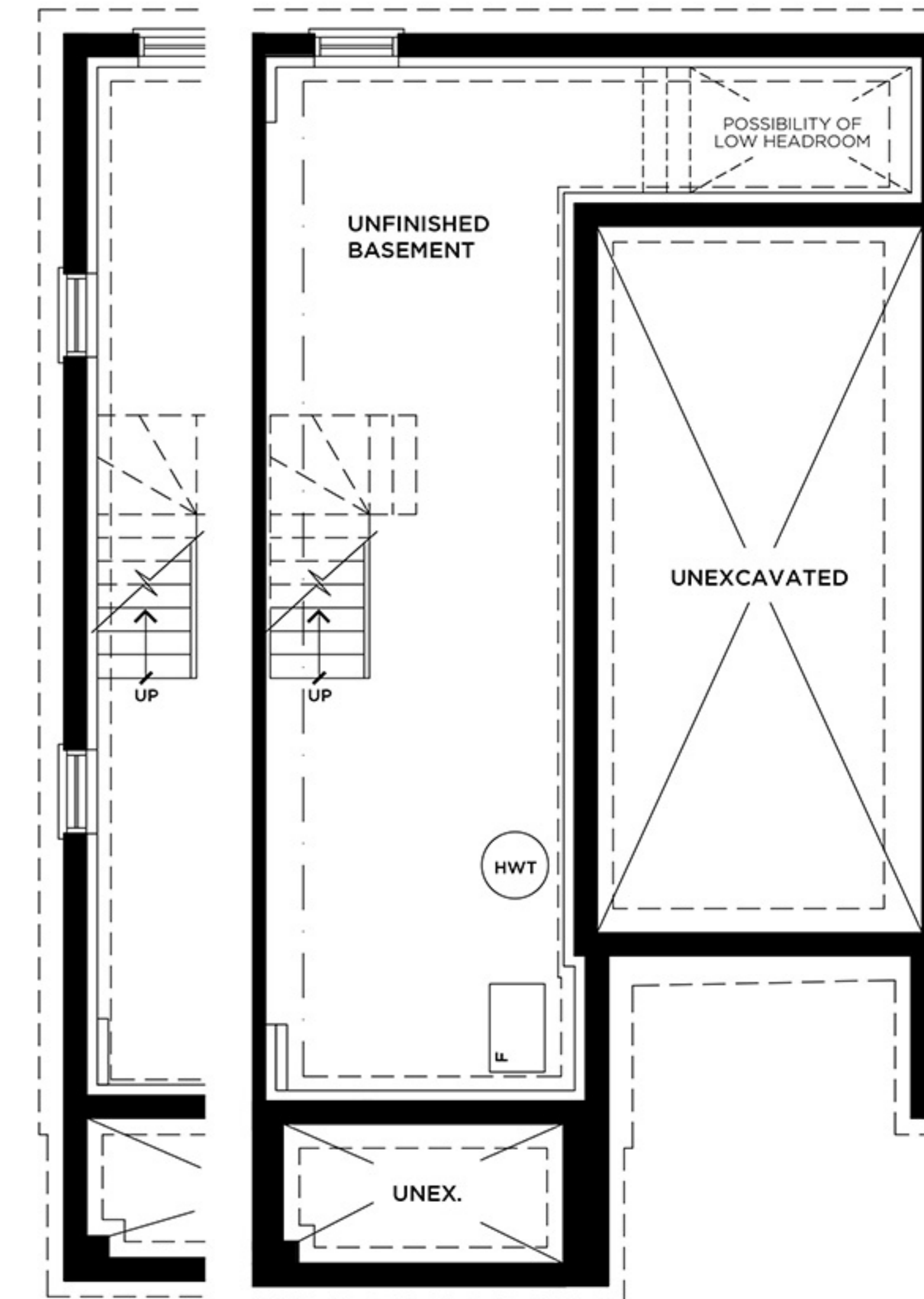
END UNIT ELEV. 'B' UNIT 18, 25 BASEMENT PLAN ELEV. 'B' UNIT 19-24
