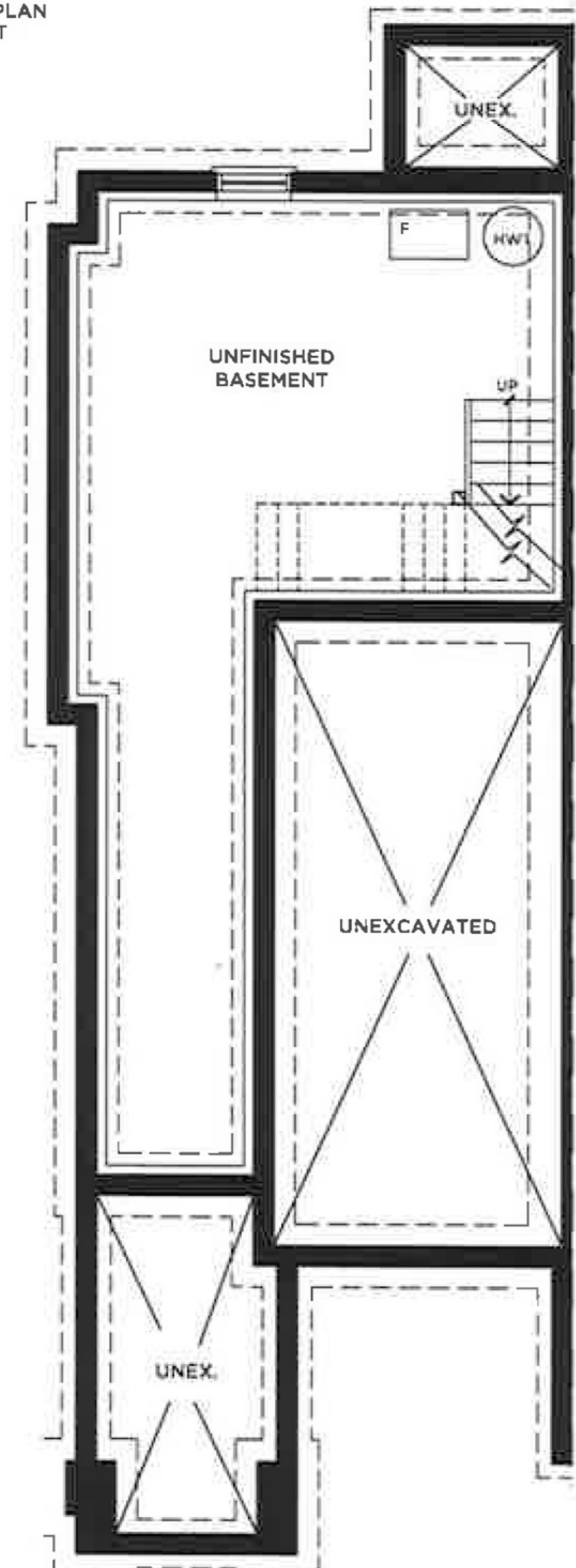
BASEMENT PLAN ELEV. 'B' END UNIT UNIT 26, 32
