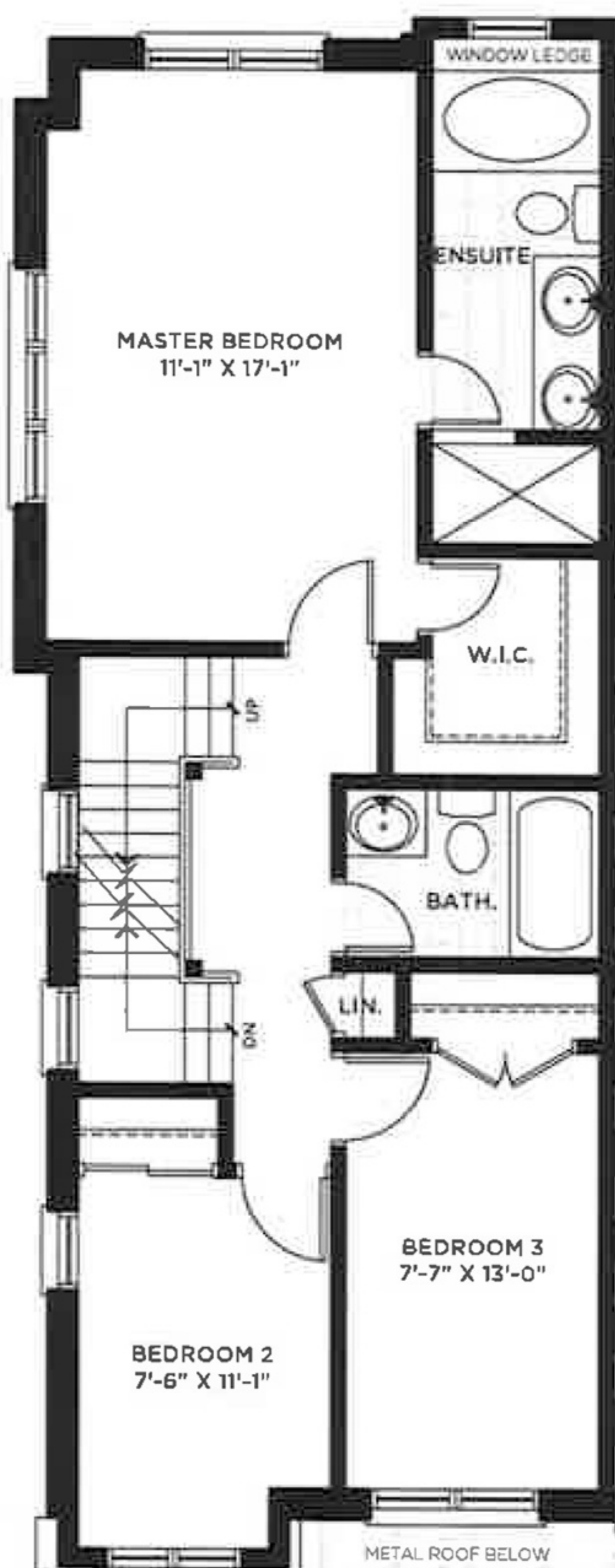
THIRD FLOOR PLAN ELEV. 'B' END UNIT UNIT 26, 32
