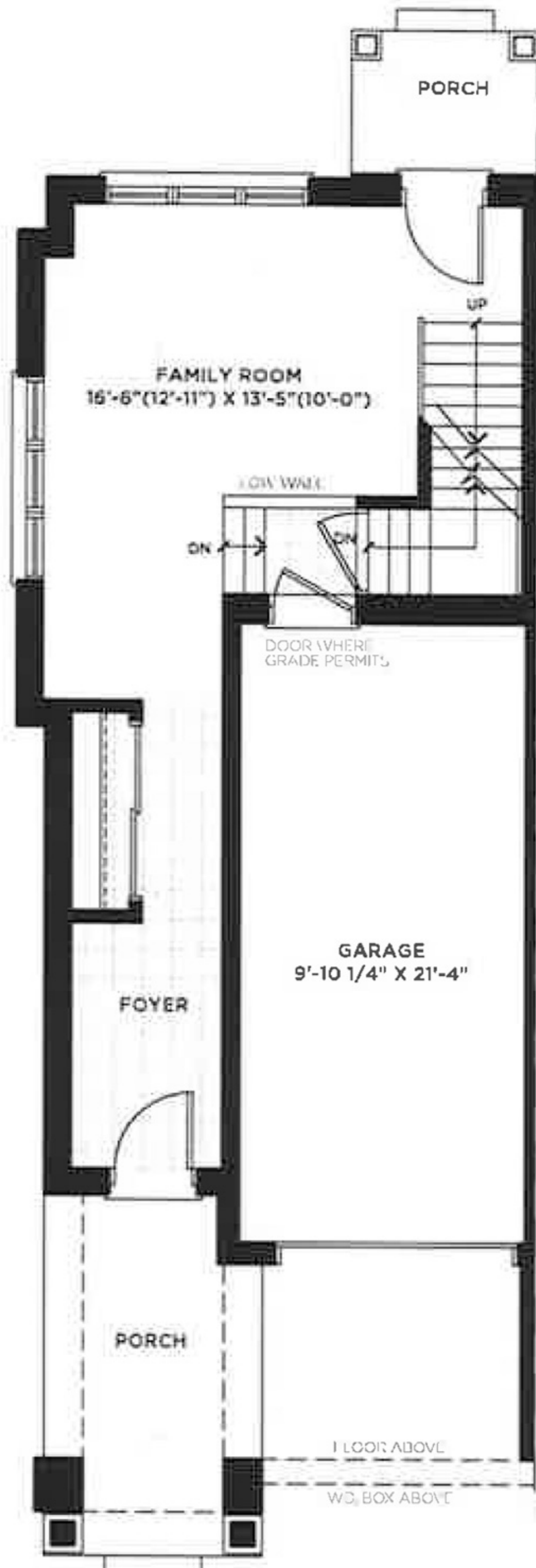
FIRST FLOOR PLAN ELEV. 'B' END UNIT UNIT 26, 32
