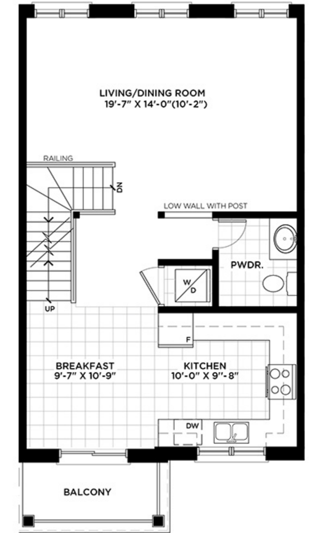
SECOND FLOOR PLAN ELEV. 'A' UNIT 10-17, 63-65
