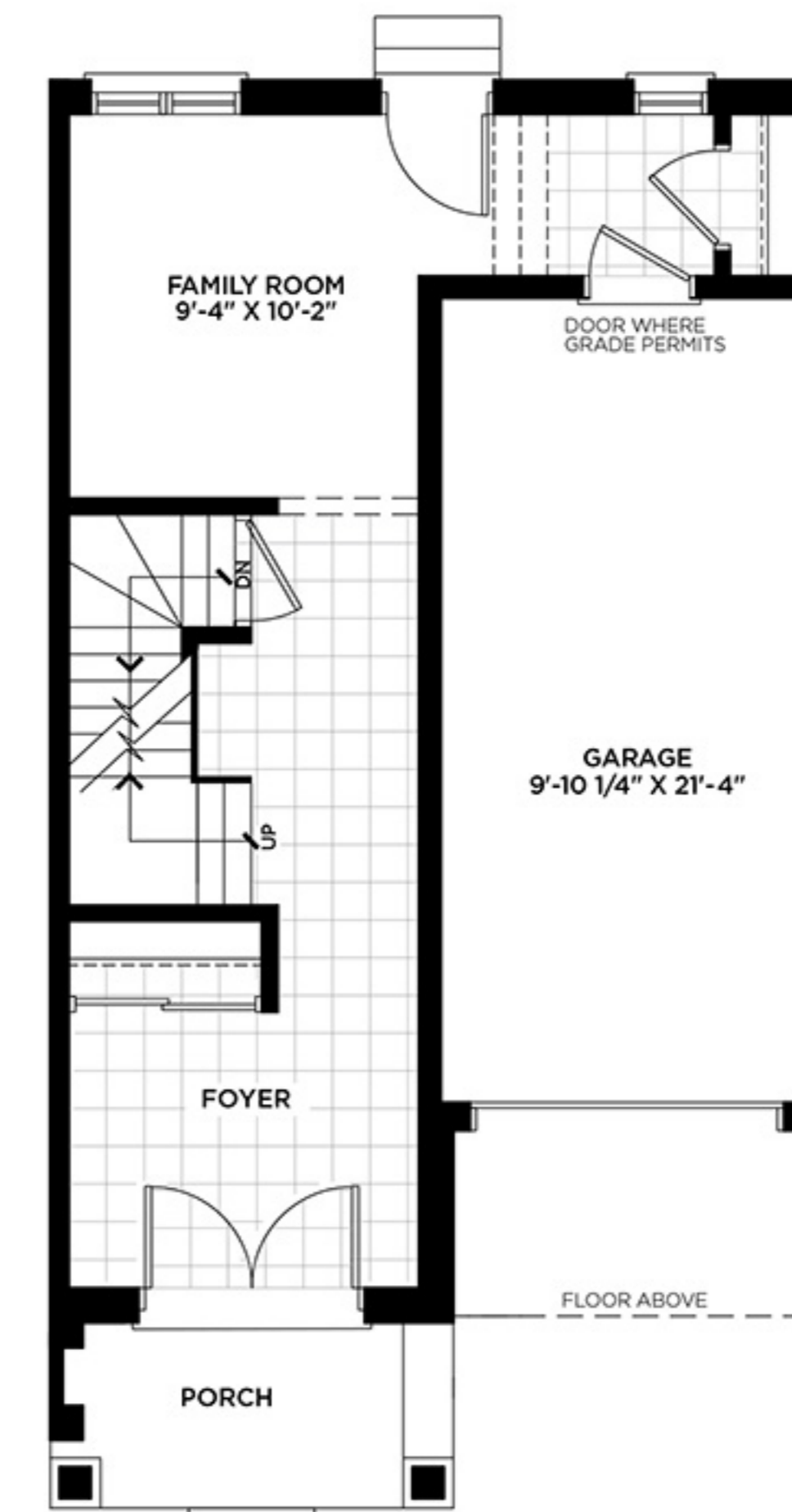
FIRST FLOOR PLAN ELEV. 'A' UNIT 10-17, 63-65
