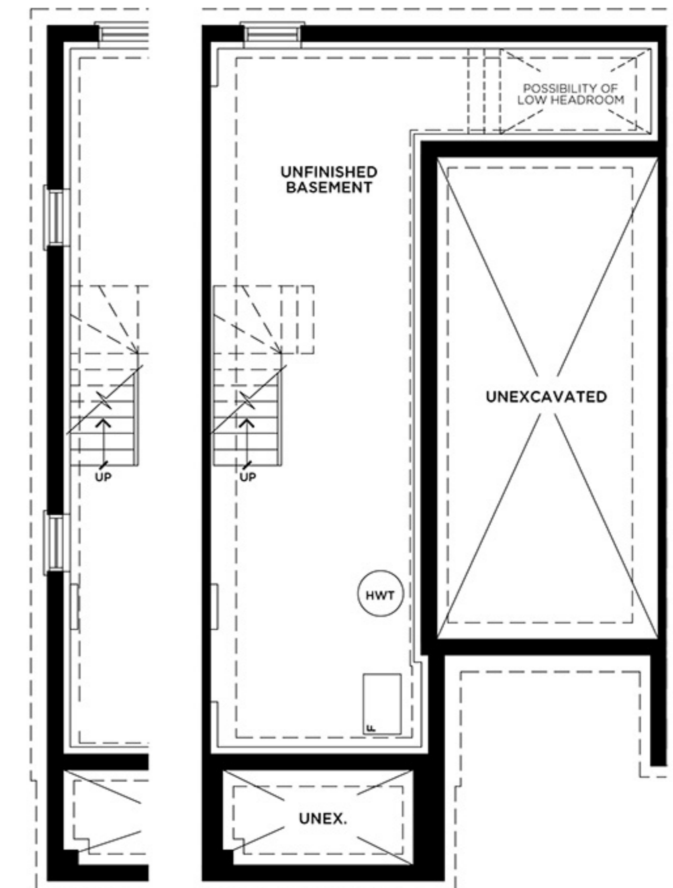
END UNIT ELEV. 'A' UNIT 10, 17, 63
